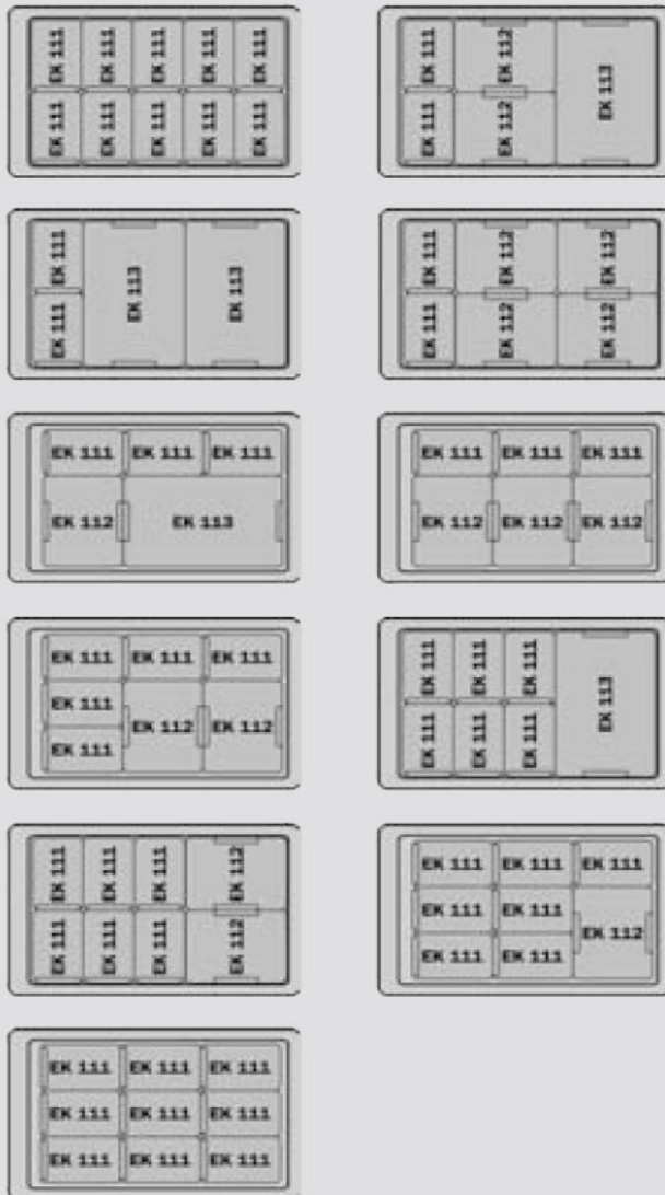
Partitioning examples with Insert boxes for LF 531, LF 532 and LF 533
